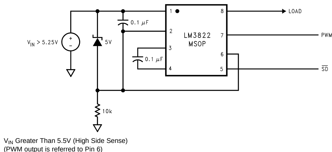
Figure 16. High Voltage Operation
